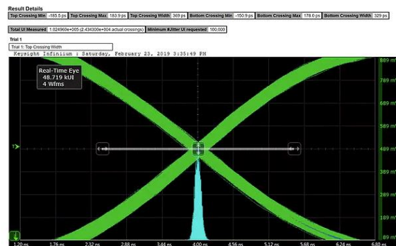
Omnia SW-8 jitter is much lower (369 ps)
