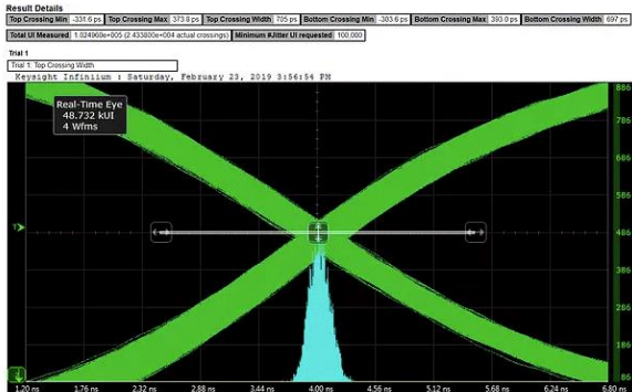
Standard Network Switch Jitter (as high as 705ps)
