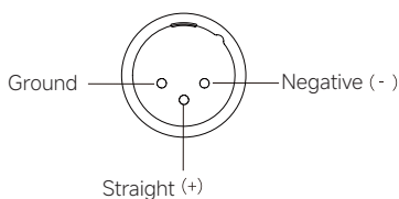
Set reverse port polarity diagram
