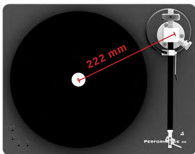
Pic. 7: Distance between spindle and pivot point
