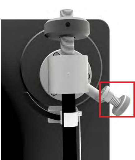
Illustration 1 (minimal antiskating)
